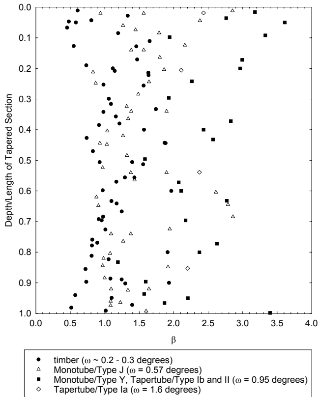
Fig. 4. Calculated \beta Values as a Function of Taper Angle.
